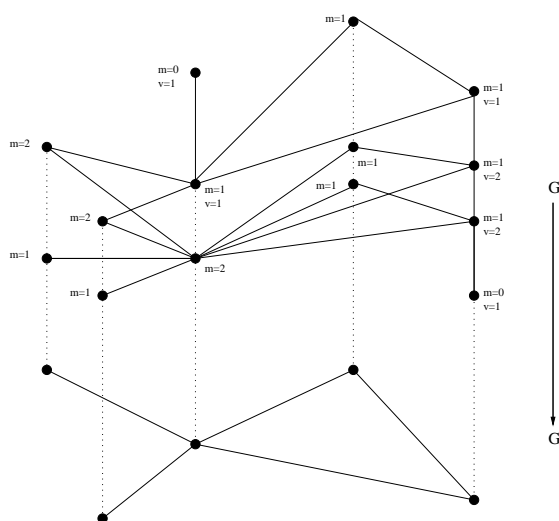
FIGURE 1. A harmonic morphism \phi : G \rightarrow G' of degree 3.
